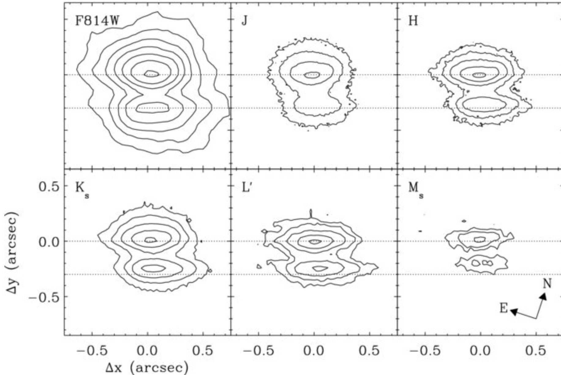
Figure 3. from Panchromatic Observations and Modeling of the HV Tau C Edge-on Disk DUCHÊNE ET AL. 2010 ApJ 712 112 doi:10.1088/0004-637X/712/1/112 https://dx.doi.org/10.1088/0004-637X/712/1/112 © 2010. The American Astronomical Society. All rights reserved.
