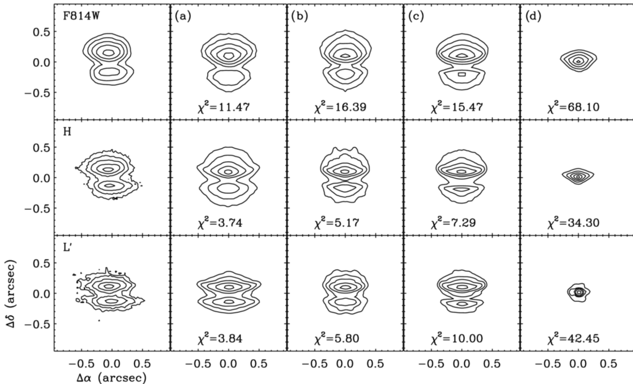
Figure 10. from Panchromatic Observations and Modeling of the HV Tau C Edge-on Disk DUCHÊNE ET AL. 2010 ApJ 712 112 doi:10.1088/0004-637X/712/1/112 https://dx.doi.org/10.1088/0004-637X/712/1/112 © 2010. The American Astronomical Society. All rights reserved.
