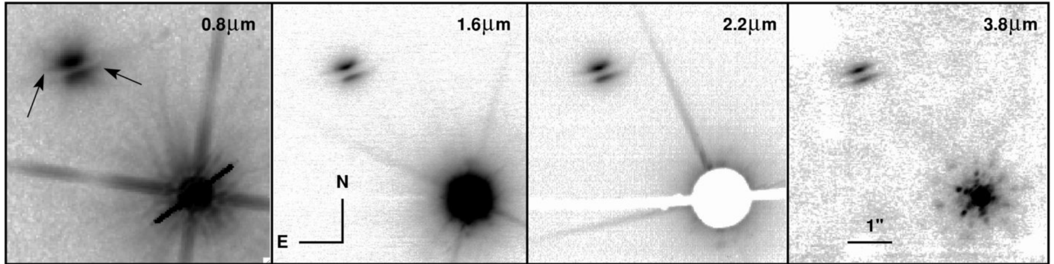
Figure 1. from Panchromatic Observations and Modeling of the HV Tau C Edge-on Disk DUCHÊNE ET AL. 2010 ApJ 712 112 doi:10.1088/0004-637X/712/1/112 https://dx.doi.org/10.1088/0004-637X/712/1/112 © 2010. The American Astronomical Society. All rights reserved.
