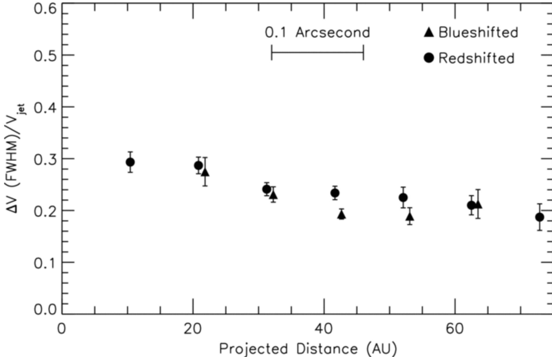
Figure 5. from Adaptive Optics Echelle Spectroscopy of [Fe II] 1.644 \mu m in the RW Aur Jet: A Narrow Slice Down the Axis of the Flow HARTIGAN & HILLENBRAND 2009 ApJ 705 1388 doi:10.1088/0004-637X/705/2/1388 https://dx.doi.org/10.1088/0004-637X/705/2/1388 © 2009. The American Astronomical Society. All rights reserved.
