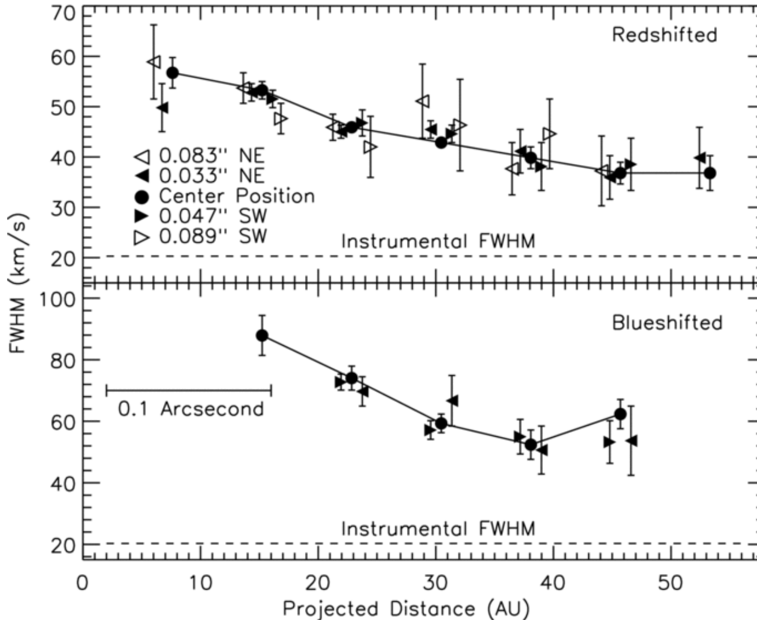
Figure 3. from Adaptive Optics Echelle Spectroscopy of [Fe II] 1.644 \mu m in the RW Aur Jet: A Narrow Slice Down the Axis of the Flow HARTIGAN & HILLENBRAND 2009 ApJ 705 1388 doi:10.1088/0004-637X/705/2/1388 https://dx.doi.org/10.1088/0004-637X/705/2/1388 © 2009. The American Astronomical Society. All rights reserved.
