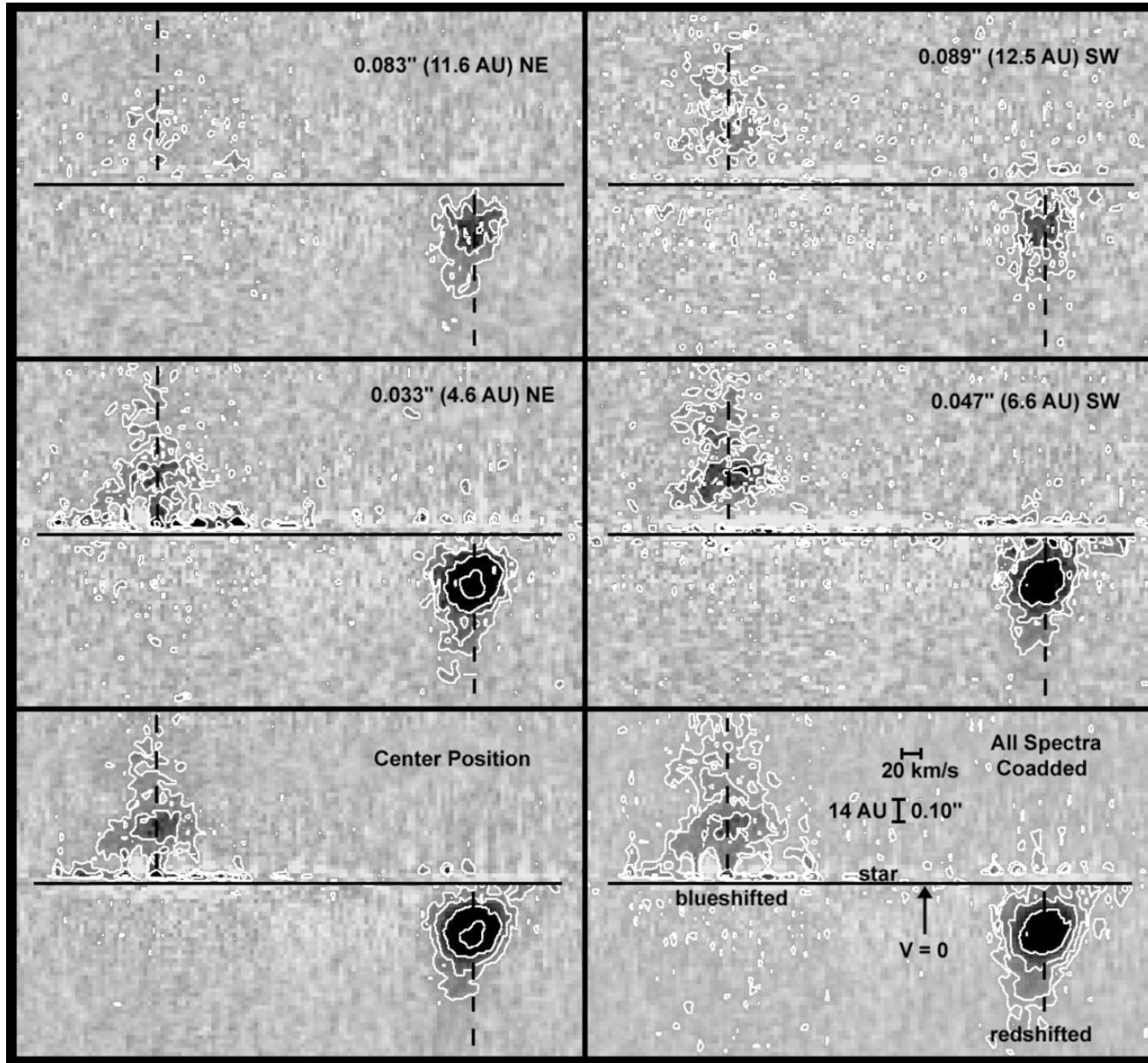
Figure 1. from Adaptive Optics Echelle Spectroscopy of [Fe II] 1.644 \mu m in the RW Aur Jet: A Narrow Slice Down the Axis of the Flow HARTIGAN & HILLENBRAND 2009 ApJ 705 1388 doi:10.1088/0004-637X/705/2/1388 https://dx.doi.org/10.1088/0004-637X/705/2/1388 © 2009. The American Astronomical Society. All rights reserved.
