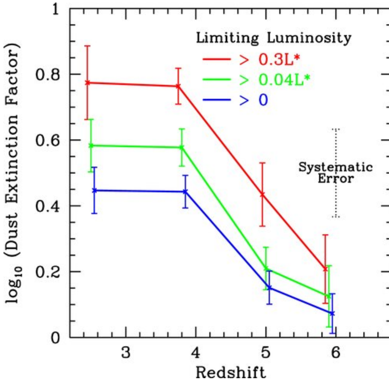
Figure 8. from UV Continuum Slope and Dust Obscuration from z = 6 to z = 2 : The Star Formation Rate Density at High Redshift BOUWENS ET AL. 2009 ApJ 705 936 doi:10.1088/0004-637X/705/1/936 https://dx.doi.org/10.1088/0004-637X/705/1/936 © 2009. The American Astronomical Society. All rights reserved.
