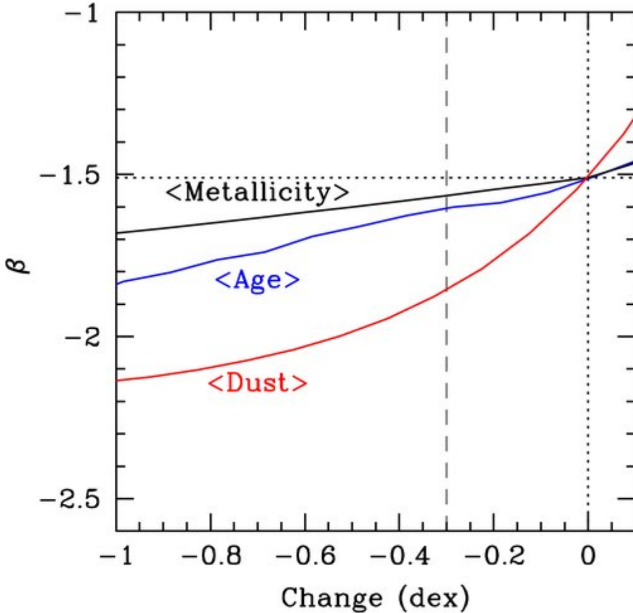
Figure 7. from UV Continuum Slope and Dust Obscuration from z = 6 to z = 2 : The Star Formation Rate Density at High Redshift BOUWENS ET AL. 2009 ApJ 705 936 doi:10.1088/0004-637X/705/1/936 https://dx.doi.org/10.1088/0004-637X/705/1/936 © 2009. The American Astronomical Society. All rights reserved.
