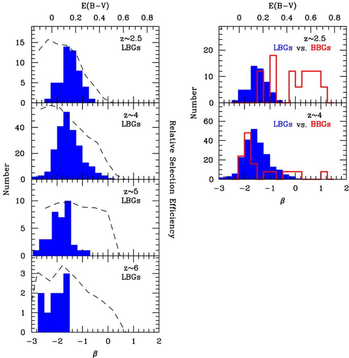
Figure 6. from UV Continuum Slope and Dust Obscuration from z \sim 6 to z \sim 2 : The Star Formation Rate Density at High Redshift BOUWENS ET AL. 2009 ApJ 705 936 doi:10.1088/0004-637X/705/1/936 https://dx.doi.org/10.1088/0004-637X/705/1/936 © 2009. The American Astronomical Society. All rights reserved.
