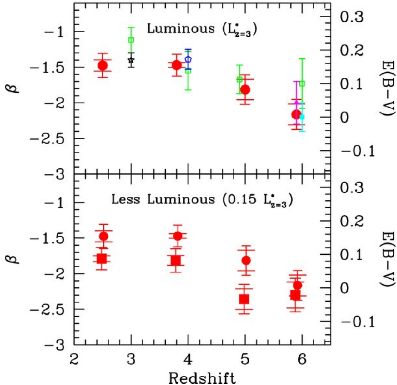
Figure 5. from UV Continuum Slope and Dust Obscuration from z = 6 to z = 2 : The Star Formation Rate Density at High Redshift BOUWENS ET AL. 2009 ApJ 705 936 doi:10.1088/0004-637X/705/1/936 https://dx.doi.org/10.1088/0004-637X/705/1/936 © 2009. The American Astronomical Society. All rights reserved.
