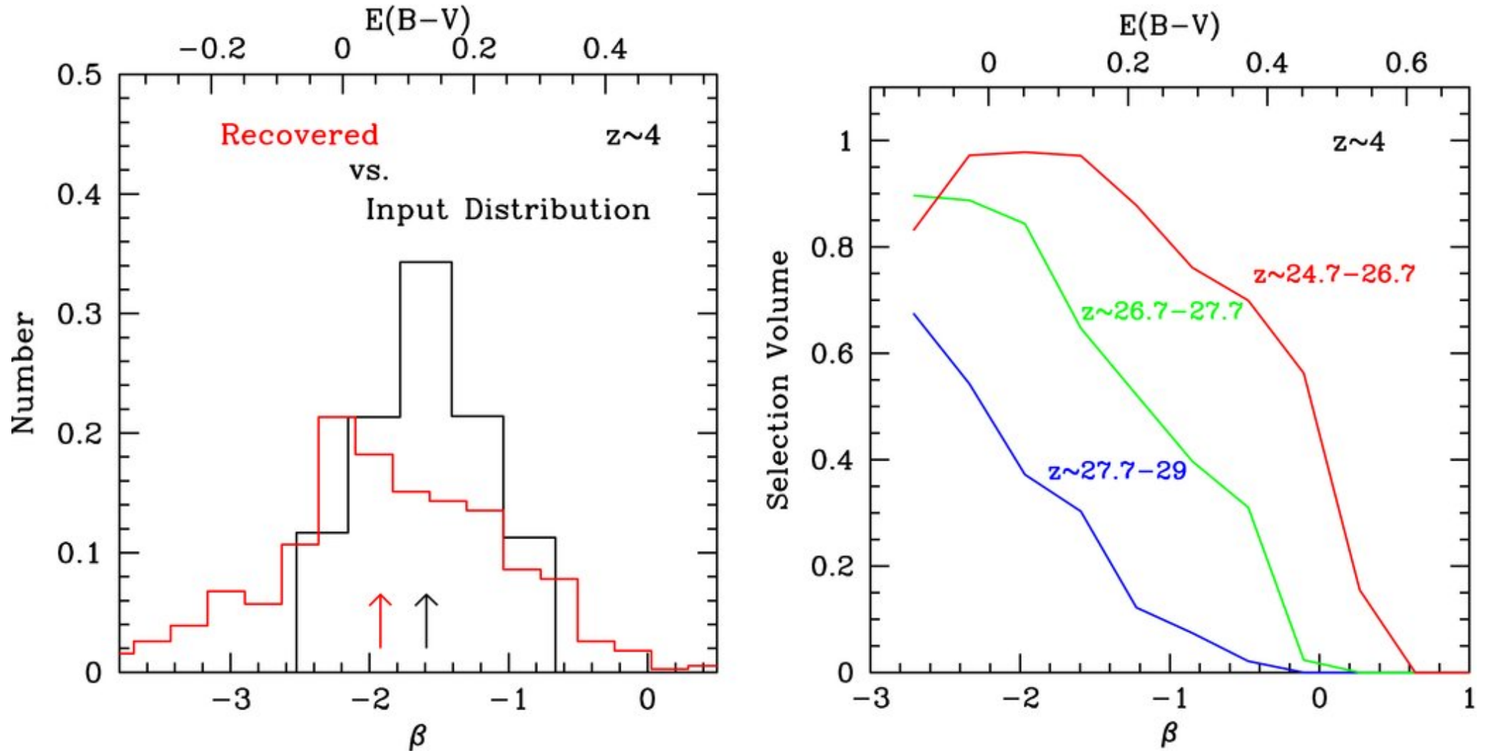
Figure 4. from UV Continuum Slope and Dust Obscuration from z \sim 6 to z \sim 2 : The Star Formation Rate Density at High Redshift BOUWENS ET AL. 2009 ApJ 705 936 doi:10.1088/0004-637X/705/1/936 https://dx.doi.org/10.1088/0004-637X/705/1/936 © 2009. The American Astronomical Society. All rights reserved.
