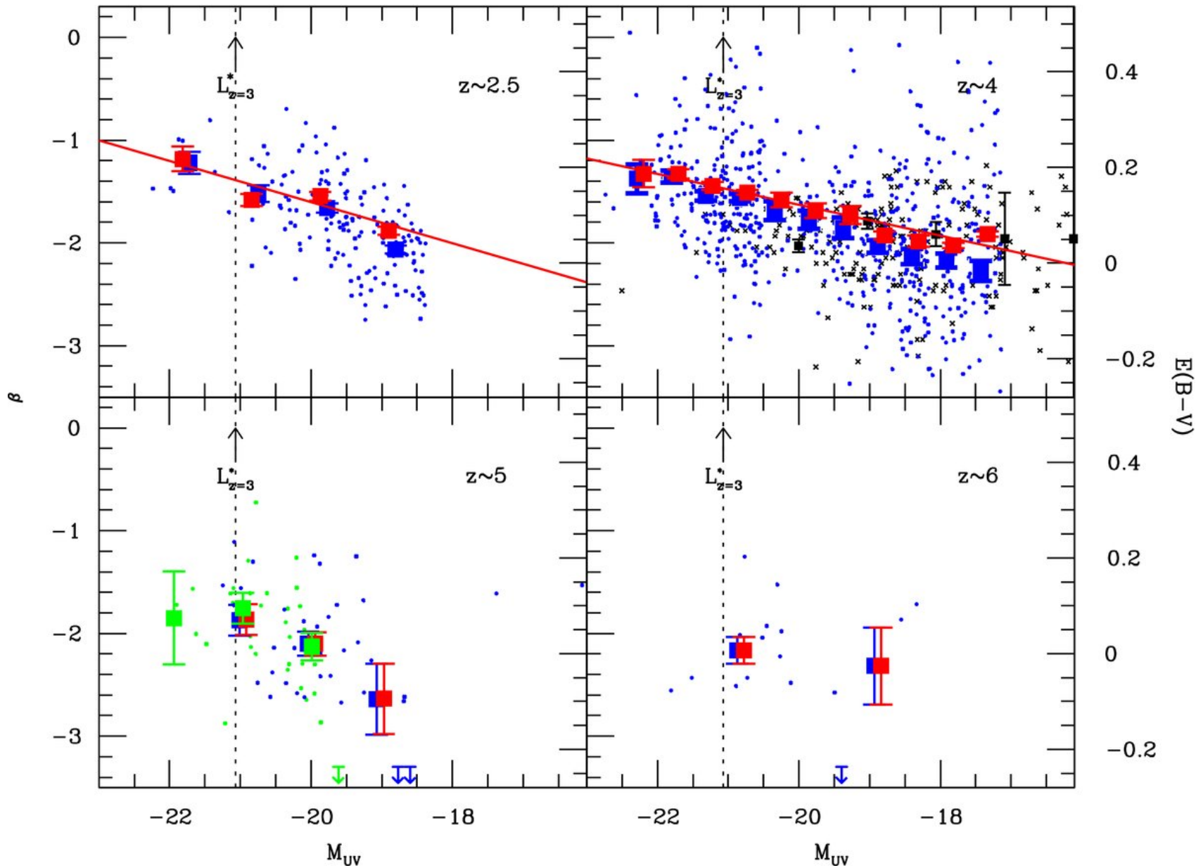
Figure 3. from UV Continuum Slope and Dust Obscuration from z \sim 6 to z \sim 2 : The Star Formation Rate Density at High Redshift BOUWENS ET AL. 2009 ApJ 705 936 doi:10.1088/0004-637X/705/1/936 https://dx.doi.org/10.1088/0004-637X/705/1/936 © 2009. The American Astronomical Society. All rights reserved.
