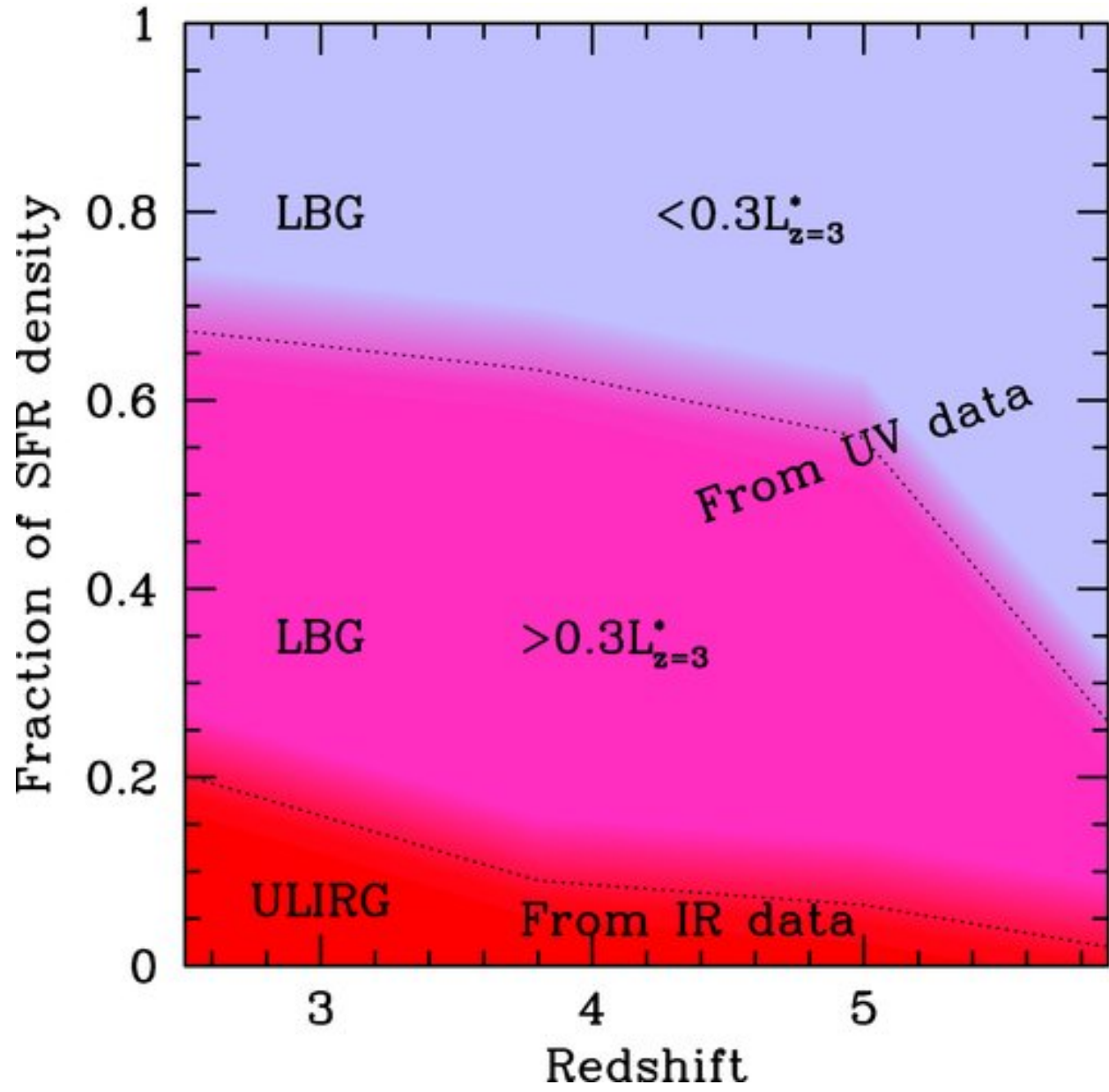
Figure 14. from UV Continuum Slope and Dust Obscuration from z = 6 to z = 2 : The Star Formation Rate Density at High Redshift BOUWENS ET AL. 2009 ApJ 705 936 doi:10.1088/0004-637X/705/1/936 https://dx.doi.org/10.1088/0004-637X/705/1/936 © 2009. The American Astronomical Society. All rights reserved.
