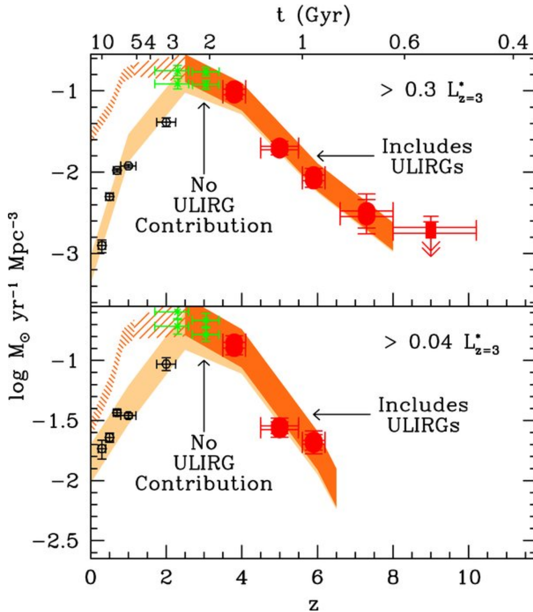
Figure 13. from UV Continuum Slope and Dust Obscuration from z = 6 to z = 2 : The Star Formation Rate Density at High Redshift BOUWENS ET AL. 2009 ApJ 705 936 doi:10.1088/0004-637X/705/1/936 https://dx.doi.org/10.1088/0004-637X/705/1/936 © 2009. The American Astronomical Society. All rights reserved.
