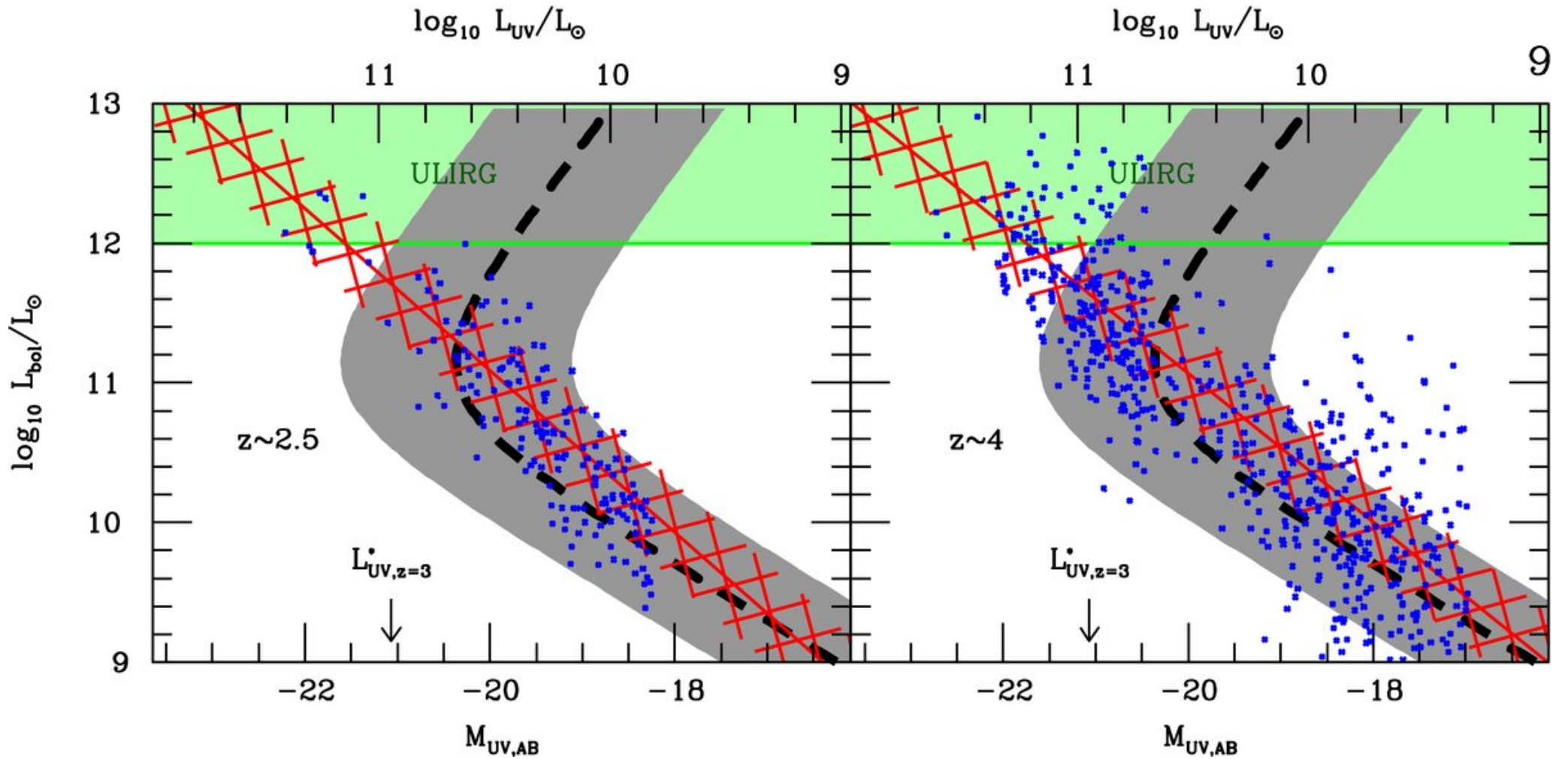
Figure 10. from UV Continuum Slope and Dust Obscuration from z \sim 6 to z \sim 2 : The Star Formation Rate Density at High Redshift BOUWENS ET AL. 2009 ApJ 705 936 doi:10.1088/0004-637X/705/1/936 https://dx.doi.org/10.1088/0004-637X/705/1/936 © 2009. The American Astronomical Society. All rights reserved.
