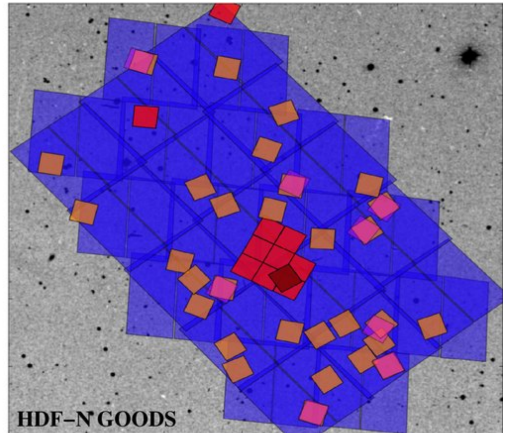
Figure 1. from UV Continuum Slope and Dust Obscuration from z = 6 to z = 2 : The Star Formation Rate Density at High Redshift BOUWENS ET AL. 2009 ApJ 705 936 doi:10.1088/0004-637X/705/1/936 https://dx.doi.org/10.1088/0004-637X/705/1/936 © 2009. The American Astronomical Society. All rights reserved.
