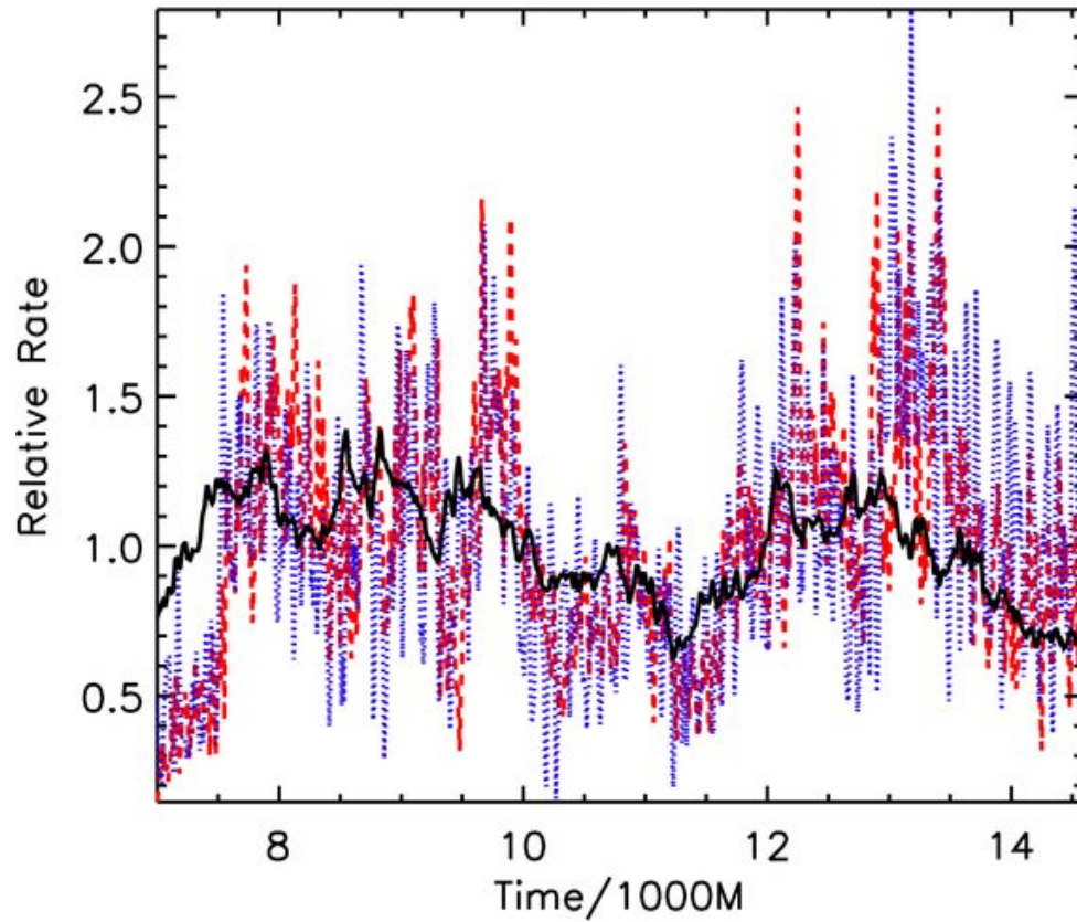
Figure 6. from GRMHD Prediction of Coronal Variability in Accreting Black Holes NOBLE & KROLIK 2009 ApJ 703 964 doi:10.1088/0004-637X/703/1/964 https://dx.doi.org/10.1088/0004-637X/703/1/964 © 2009. The American Astronomical Society. All rights reserved.
