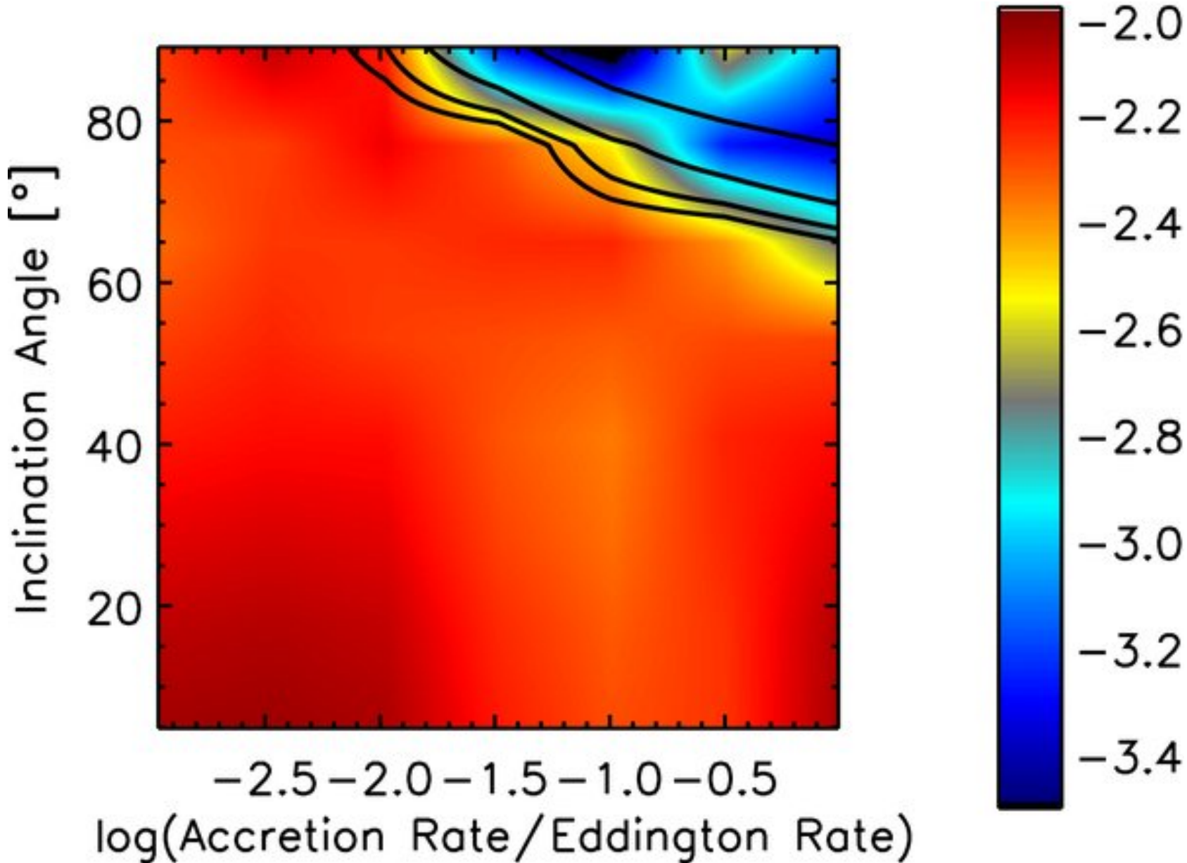
Figure 5. from GRMHD Prediction of Coronal Variability in Accreting Black Holes NOBLE & KROLIK 2009 ApJ 703 964 doi:10.1088/0004-637X/703/1/964 https://dx.doi.org/10.1088/0004-637X/703/1/964 © 2009. The American Astronomical Society. All rights reserved.
