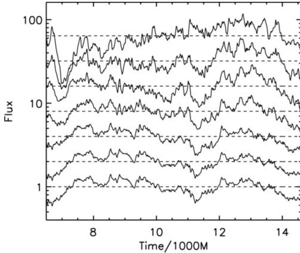
Figure 4. from GRMHD Prediction of Coronal Variability in Accreting Black Holes NOBLE & KROLIK 2009 ApJ 703 964 doi:10.1088/0004-637X/703/1/964 https://dx.doi.org/10.1088/0004-637X/703/1/964 © 2009. The American Astronomical Society. All rights reserved.
