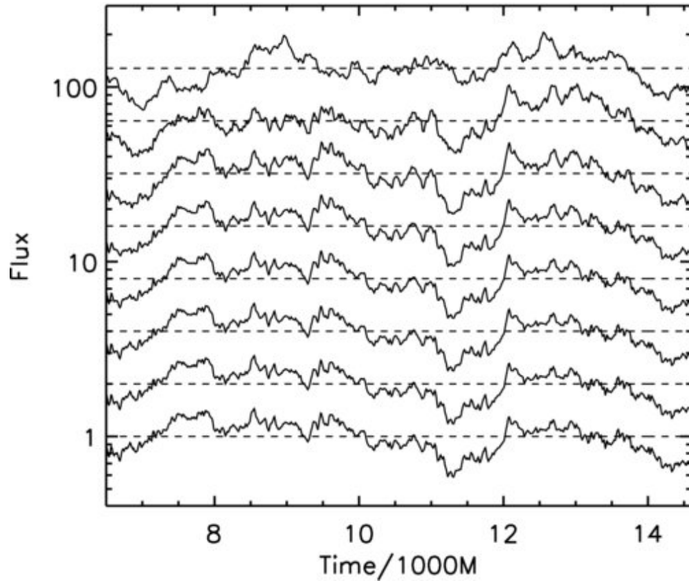
Figure 3. from GRMHD Prediction of Coronal Variability in Accreting Black Holes NOBLE & KROLIK 2009 ApJ 703 964 doi:10.1088/0004-637X/703/1/964 https://dx.doi.org/10.1088/0004-637X/703/1/964 © 2009. The American Astronomical Society. All rights reserved.
