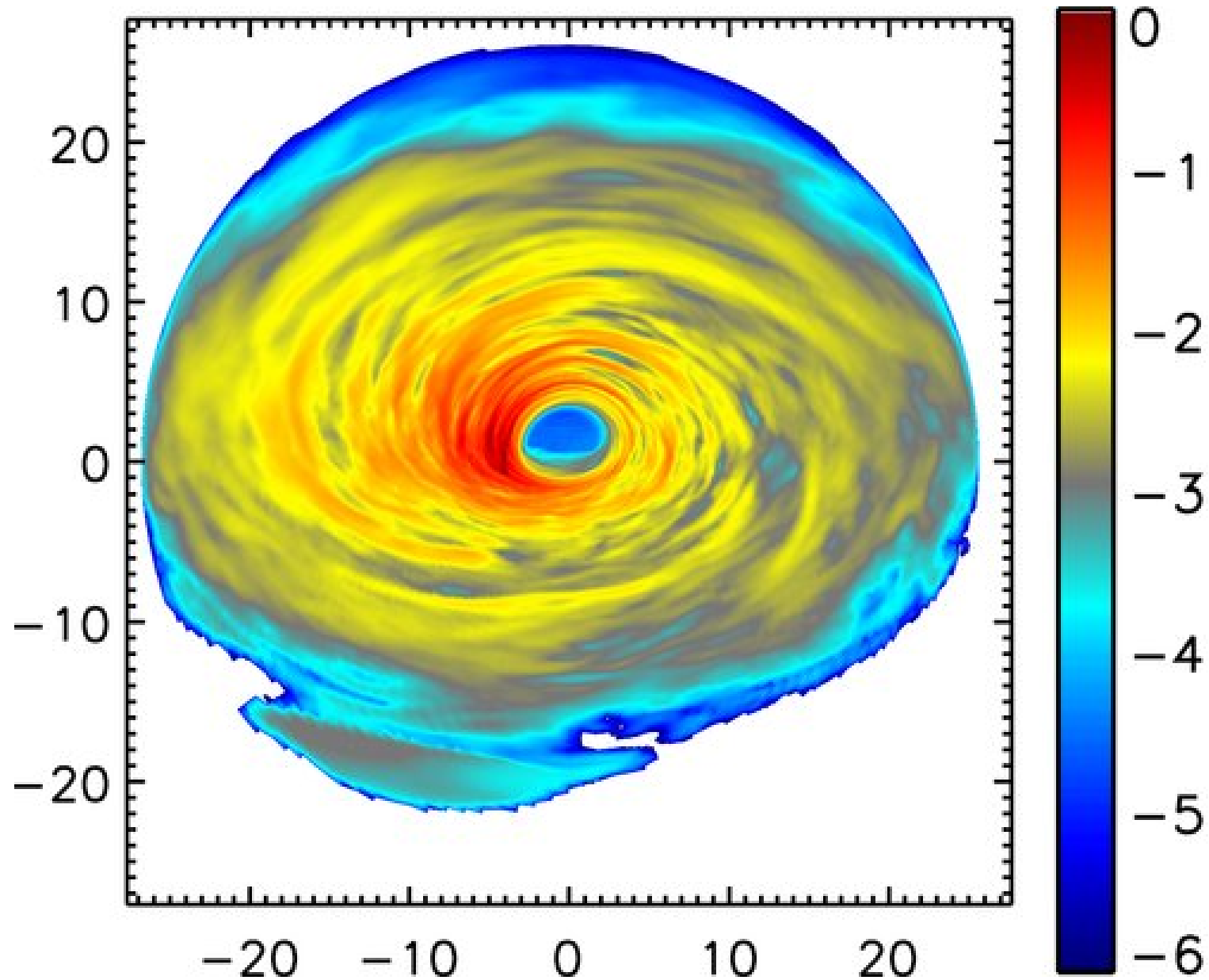
Figure 2. from GRMHD Prediction of Coronal Variability in Accreting Black Holes NOBLE & KROLIK 2009 ApJ 703 964 doi:10.1088/0004-637X/703/1/964 https://dx.doi.org/10.1088/0004-637X/703/1/964 © 2009. The American Astronomical Society. All rights reserved.
