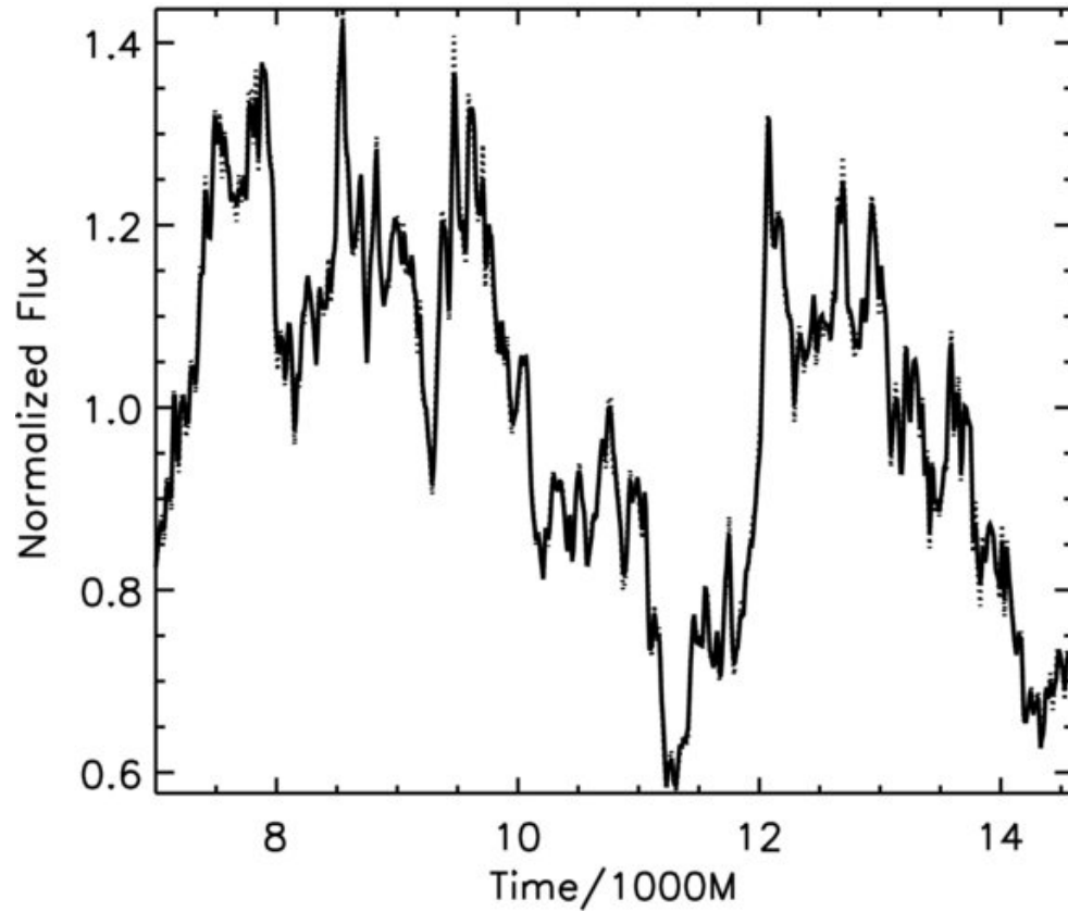
Figure 10. from GRMHD Prediction of Coronal Variability in Accreting Black Holes NOBLE & KROLIK 2009 ApJ 703 964 doi:10.1088/0004-637X/703/1/964 https://dx.doi.org/10.1088/0004-637X/703/1/964 © 2009. The American Astronomical Society. All rights reserved.
