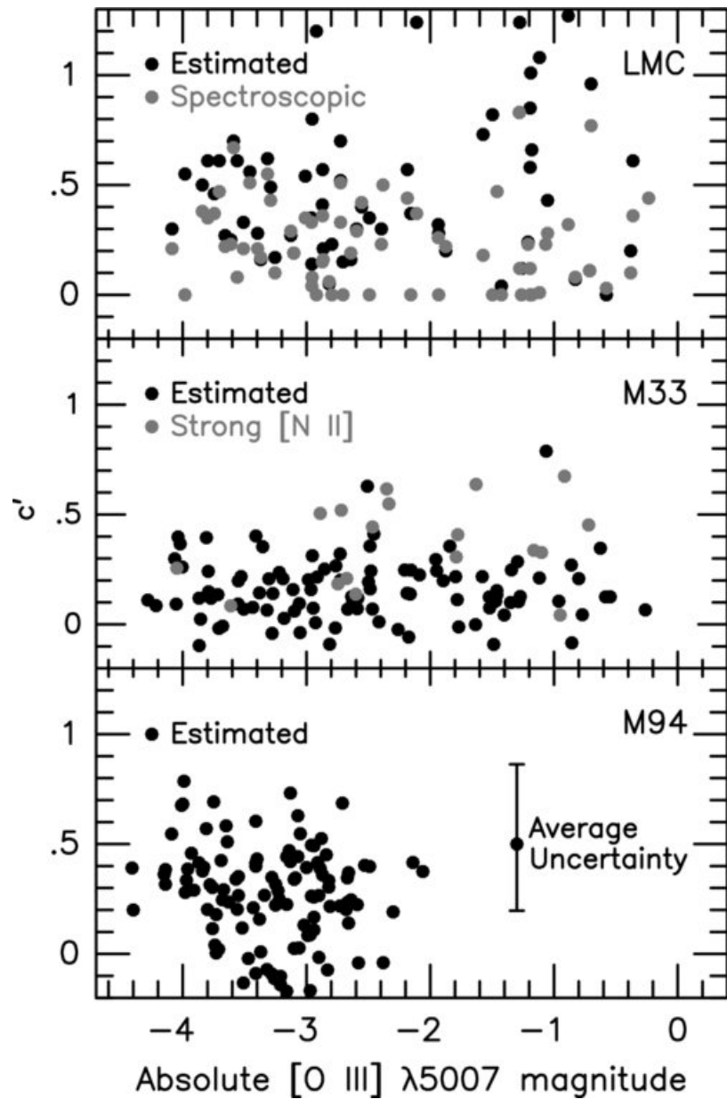
Figure 6. from Planetary Nebulae in Face-On Spiral Galaxies. II. Planetary Nebula Spectroscopy HERRMANN & CIARDULLO 2009 ApJ 703 894 doi:10.1088/0004-637X/703/1/894 https://dx.doi.org/10.1088/0004-637X/703/1/894 © 2009. The American Astronomical Society. All rights reserved.
