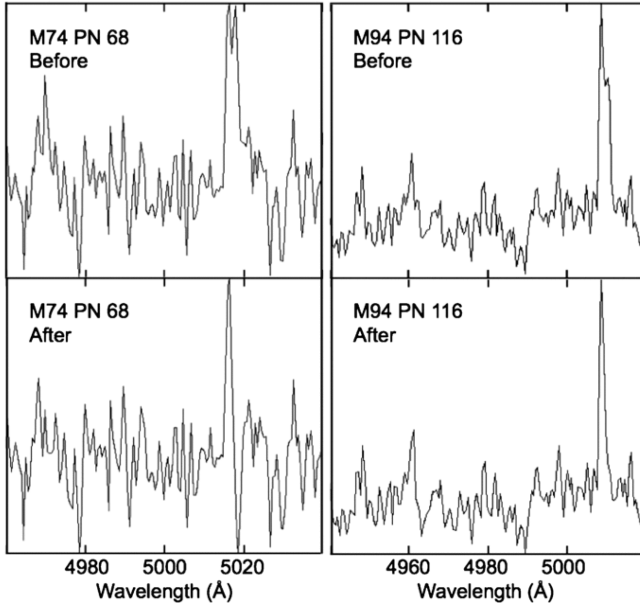
Figure 3. from Planetary Nebulae in Face-On Spiral Galaxies. II. Planetary Nebula Spectroscopy HERRMANN & CIARDULLO 2009 ApJ 703 894 doi:10.1088/0004-637X/703/1/894 https://dx.doi.org/10.1088/0004-637X/703/1/894 © 2009. The American Astronomical Society. All rights reserved.
