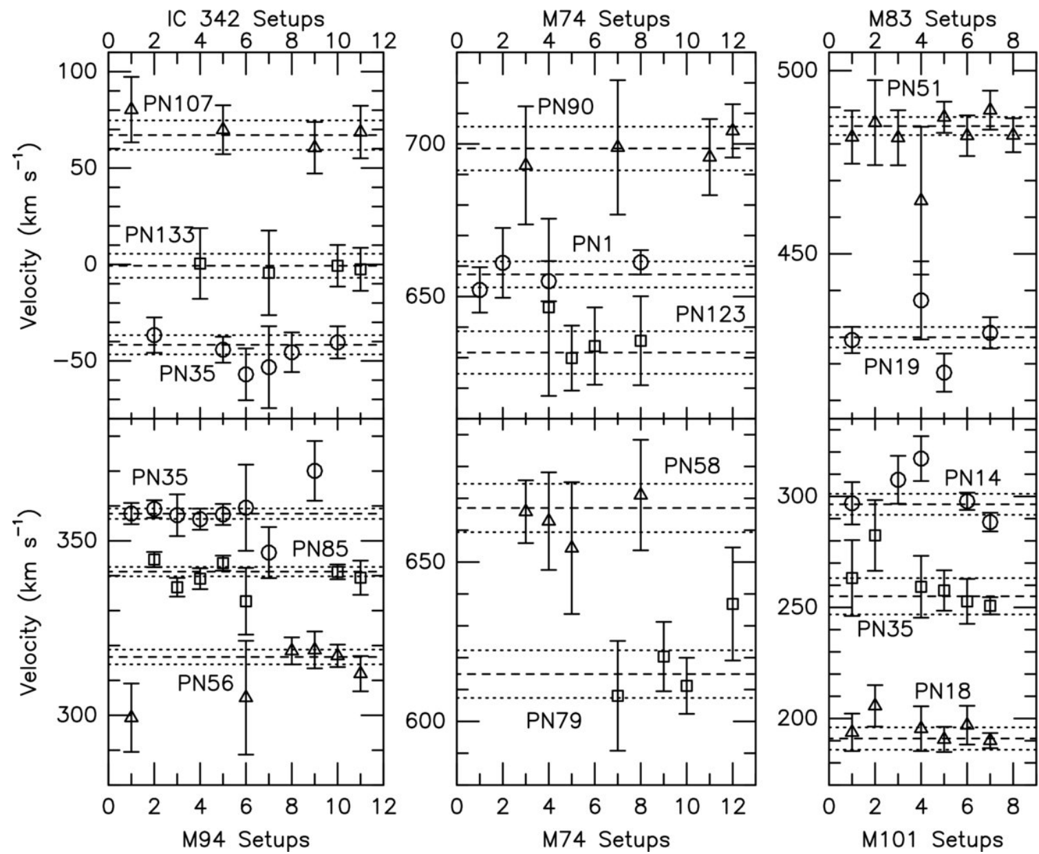
Figure 2. from Planetary Nebulae in Face-On Spiral Galaxies. II. Planetary Nebula Spectroscopy HERRMANN & CIARDULLO 2009 ApJ 703 894 doi:10.1088/0004-637X/703/1/894 https://dx.doi.org/10.1088/0004-637X/703/1/894 © 2009. The American Astronomical Society. All rights reserved.
