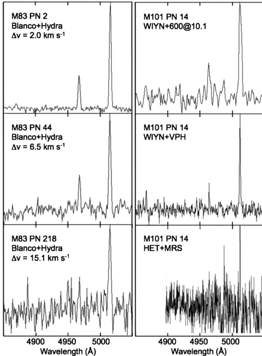
Figure 1. from Planetary Nebulae in Face-On Spiral Galaxies. II. Planetary Nebula Spectroscopy HERRMANN & CIARDULLO 2009 ApJ 703 894 doi:10.1088/0004-637X/703/1/894 https://dx.doi.org/10.1088/0004-637X/703/1/894 © 2009. The American Astronomical Society. All rights reserved.
