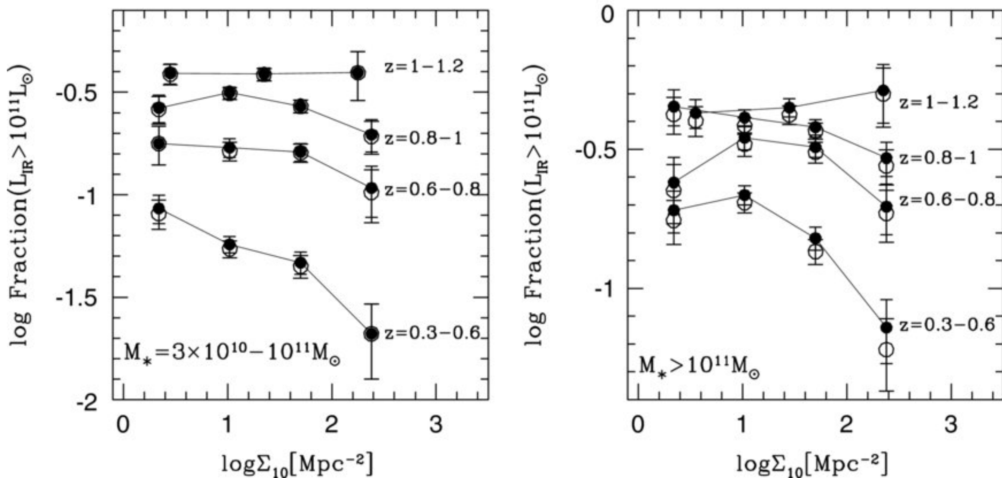
Figure 6. from Obscured Star Formation and Environment in the COSMOS Field FERUGLIO ET AL. 2010 ApJ 721 607 doi:10.1088/0004-637X/721/1/607 https://dx.doi.org/10.1088/0004-637X/721/1/607 © 2010. The American Astronomical Society. All rights reserved.
