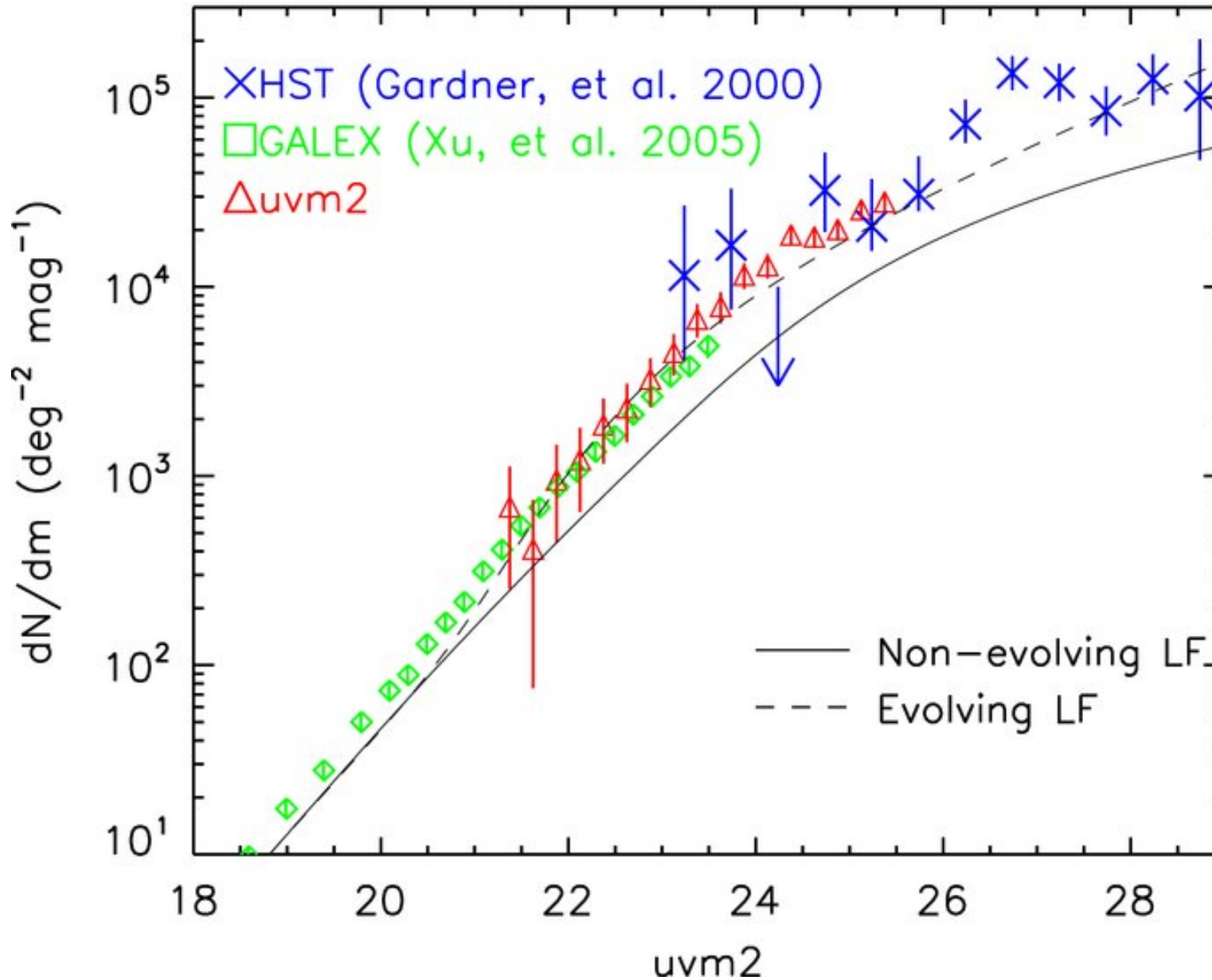
Figure 4. from Ultraviolet Number Counts of Galaxies from Swift Ultraviolet/Optical Telescope Deep Imaging of the Chandra Deep Field South HOVERSTEN ET AL. 2009 ApJ 705 1462 doi:10.1088/0004-637X/705/2/1462 https://dx.doi.org/10.1088/0004-637X/705/2/1462 © 2009. The American Astronomical Society. All rights reserved.
