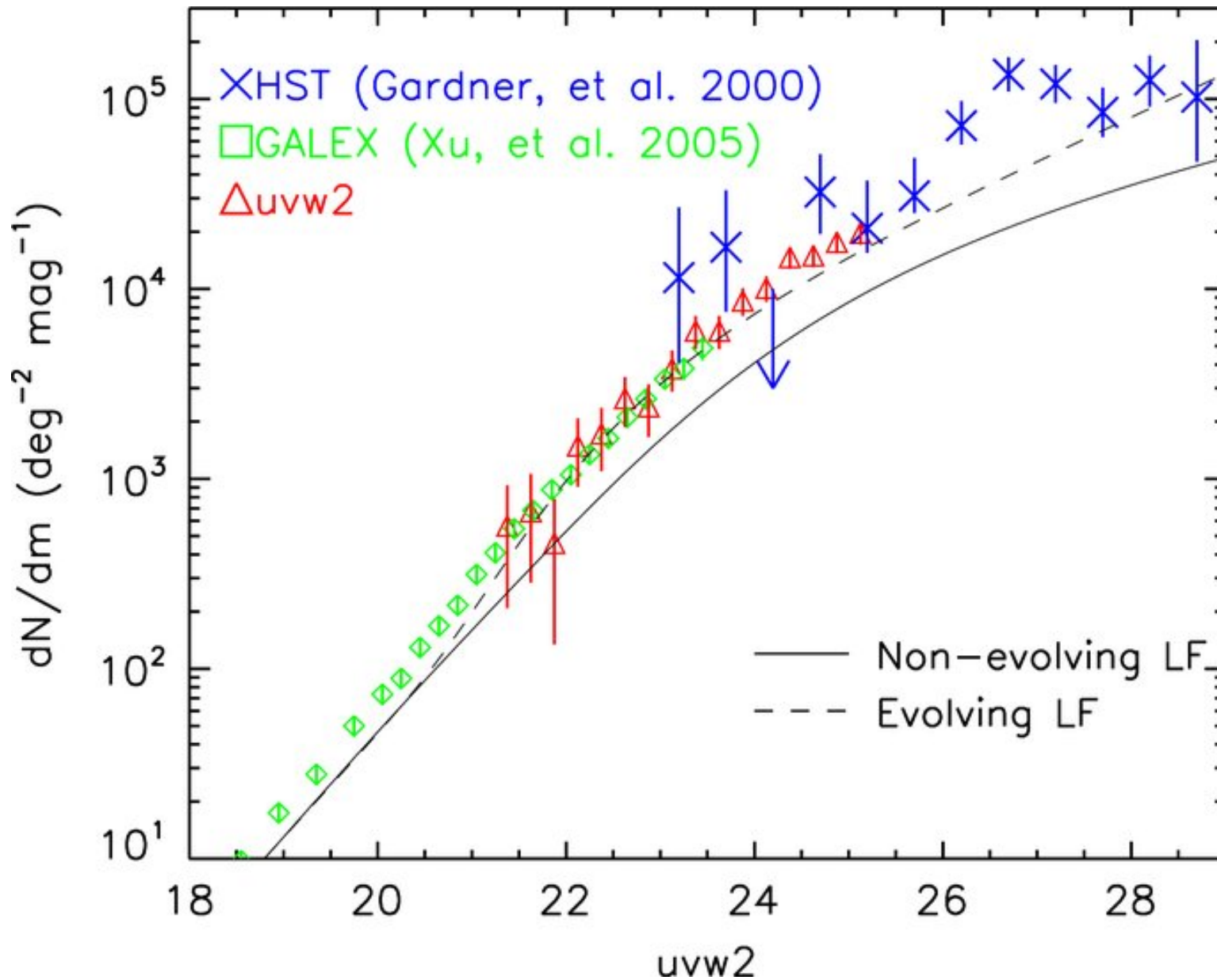
Figure 3. from Ultraviolet Number Counts of Galaxies from Swift Ultraviolet/Optical Telescope Deep Imaging of the Chandra Deep Field South HOVERSTEN ET AL. 2009 ApJ 705 1462 doi:10.1088/0004-637X/705/2/1462 https://dx.doi.org/10.1088/0004-637X/705/2/1462 © 2009. The American Astronomical Society. All rights reserved.
