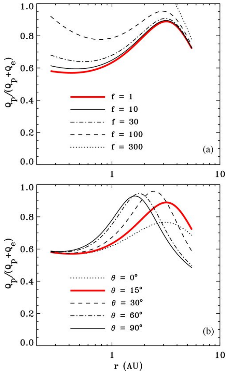
Figure 4. from Empirical Constraints on Proton and Electron Heating in the Fast Solar Wind CRANMER ET AL. 2009 ApJ 702 1604 doi:10.1088/0004-637X/702/2/1604 https://dx.doi.org/10.1088/0004-637X/702/2/1604
