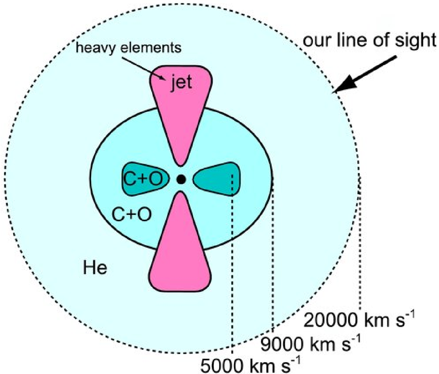
Figure 7. from Nebular Phase Observations of the Type Ib Supernova 2008D/X-ray Transient 080109: Side-viewed Bipolar Explosion TANAKA ET AL. 2009 ApJ 700 1680 doi:10.1088/0004-637X/700/2/1680 https://dx.doi.org/10.1088/0004-637X/700/2/1680 © 2009. The American Astronomical Society. All rights reserved.
