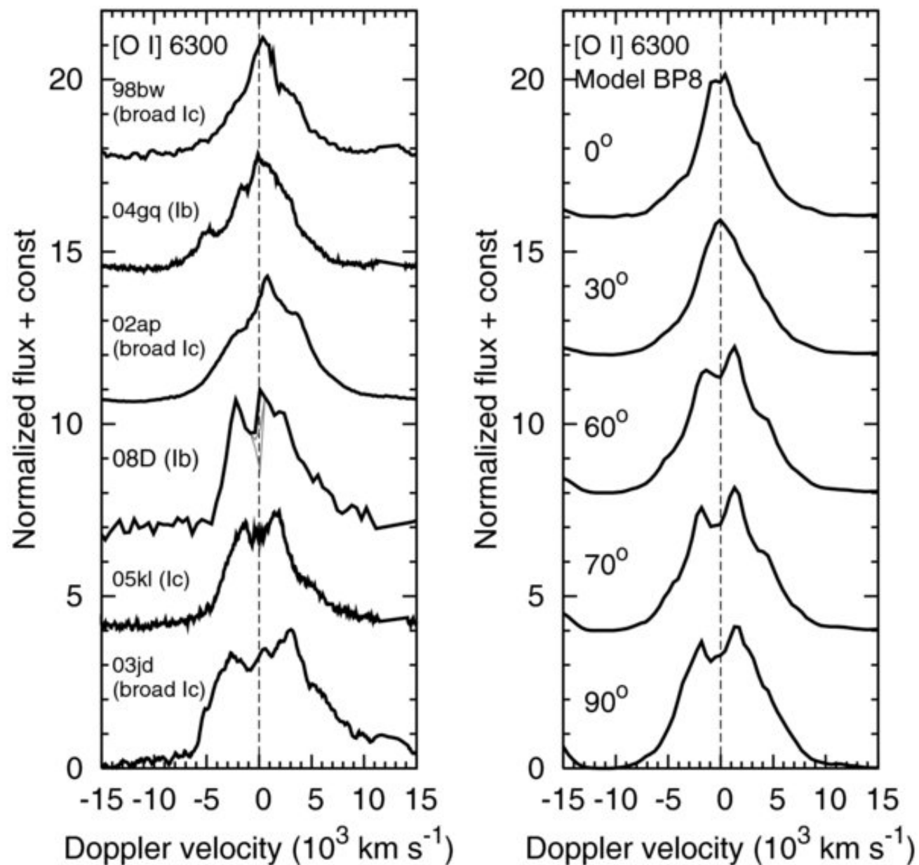
Figure 6. from Nebular Phase Observations of the Type Ib Supernova 2008D/X-ray Transient 080109: Side-viewed Bipolar Explosion TANAKA ET AL. 2009 ApJ 700 1680 doi:10.1088/0004-637X/700/2/1680 https://dx.doi.org/10.1088/0004-637X/700/2/1680 © 2009. The American Astronomical Society. All rights reserved.
