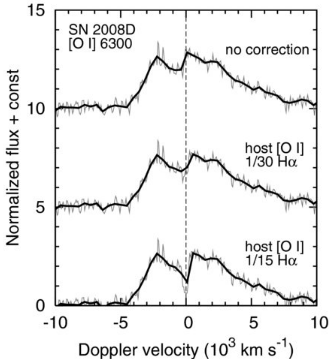
Figure 5. from Nebular Phase Observations of the Type Ib Supernova 2008D/X-ray Transient 080109: Side-viewed Bipolar Explosion TANAKA ET AL. 2009 ApJ 700 1680 doi:10.1088/0004-637X/700/2/1680 https://dx.doi.org/10.1088/0004-637X/700/2/1680 © 2009. The American Astronomical Society. All rights reserved.
