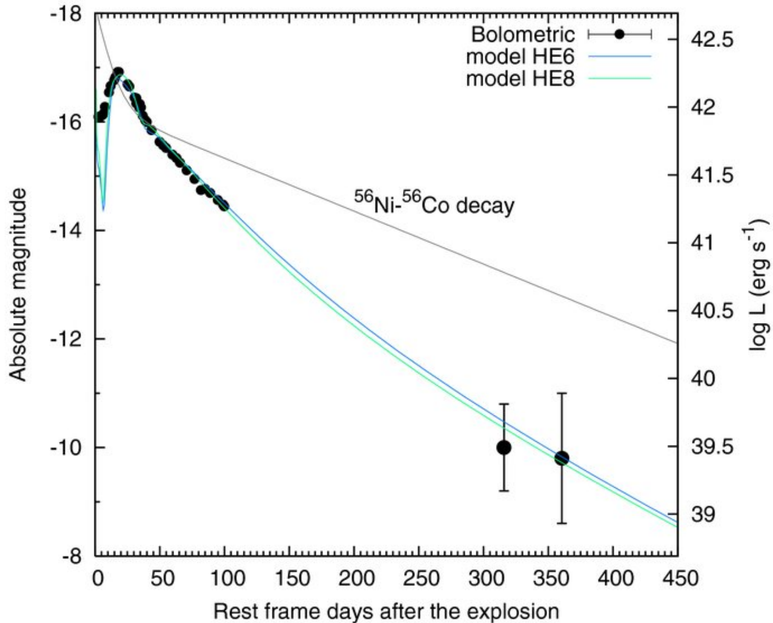
Figure 3. from Nebular Phase Observations of the Type Ib Supernova 2008D/X-ray Transient 080109: Side-viewed Bipolar Explosion TANAKA ET AL. 2009 ApJ 700 1680 doi:10.1088/0004-637X/700/2/1680 https://dx.doi.org/10.1088/0004-637X/700/2/1680 © 2009. The American Astronomical Society. All rights reserved.
