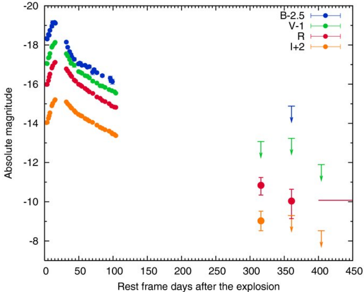
Figure 2. from Nebular Phase Observations of the Type Ib Supernova 2008D/X-ray Transient 080109: Side-viewed Bipolar Explosion TANAKA ET AL. 2009 ApJ 700 1680 doi:10.1088/0004-637X/700/2/1680 https://dx.doi.org/10.1088/0004-637X/700/2/1680 © 2009. The American Astronomical Society. All rights reserved.
