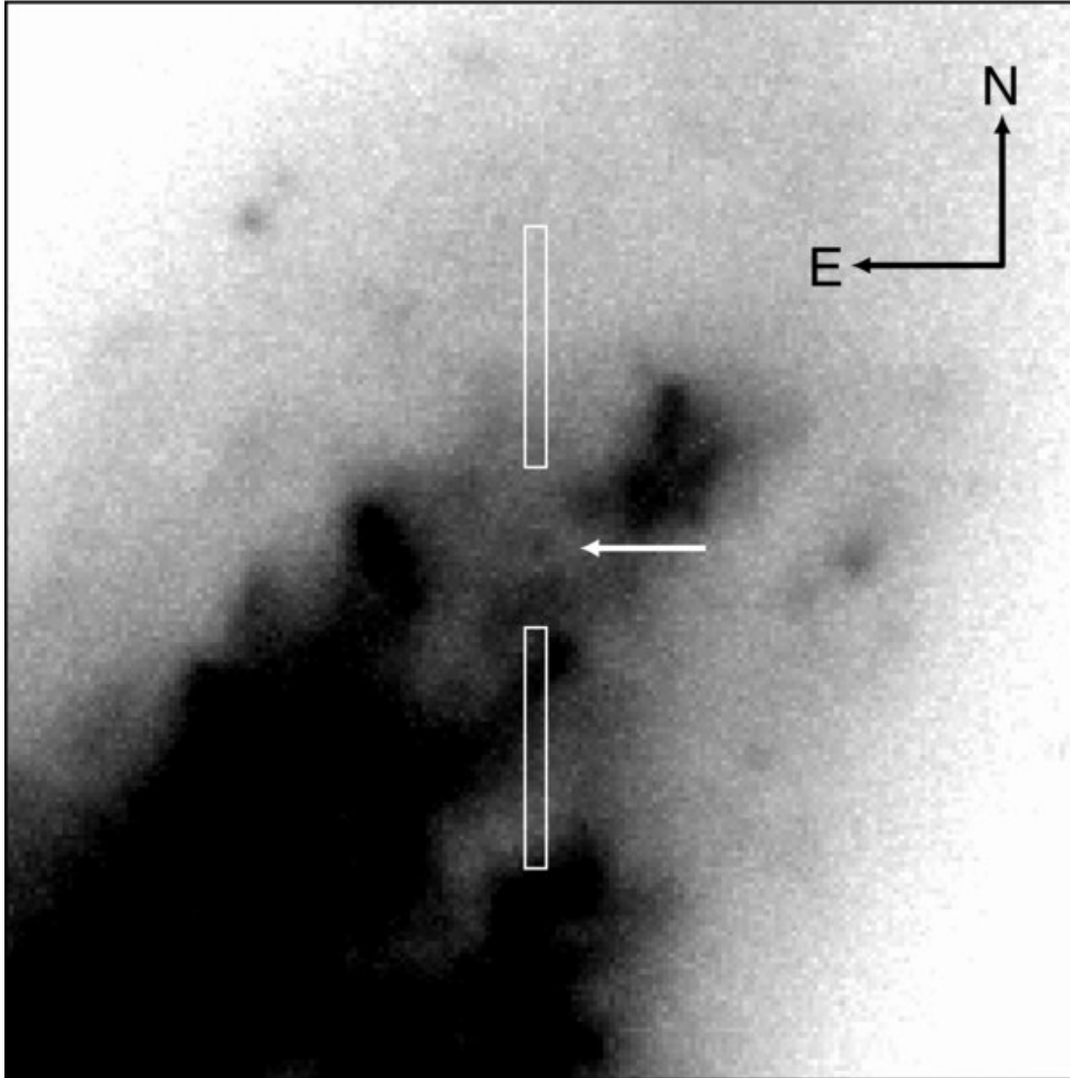
Figure 1. from Nebular Phase Observations of the Type Ib Supernova 2008D/X-ray Transient 080109: Side-viewed Bipolar Explosion TANAKA ET AL. 2009 ApJ 700 1680 doi:10.1088/0004-637X/700/2/1680 https://dx.doi.org/10.1088/0004-637X/700/2/1680 © 2009. The American Astronomical Society. All rights reserved.
