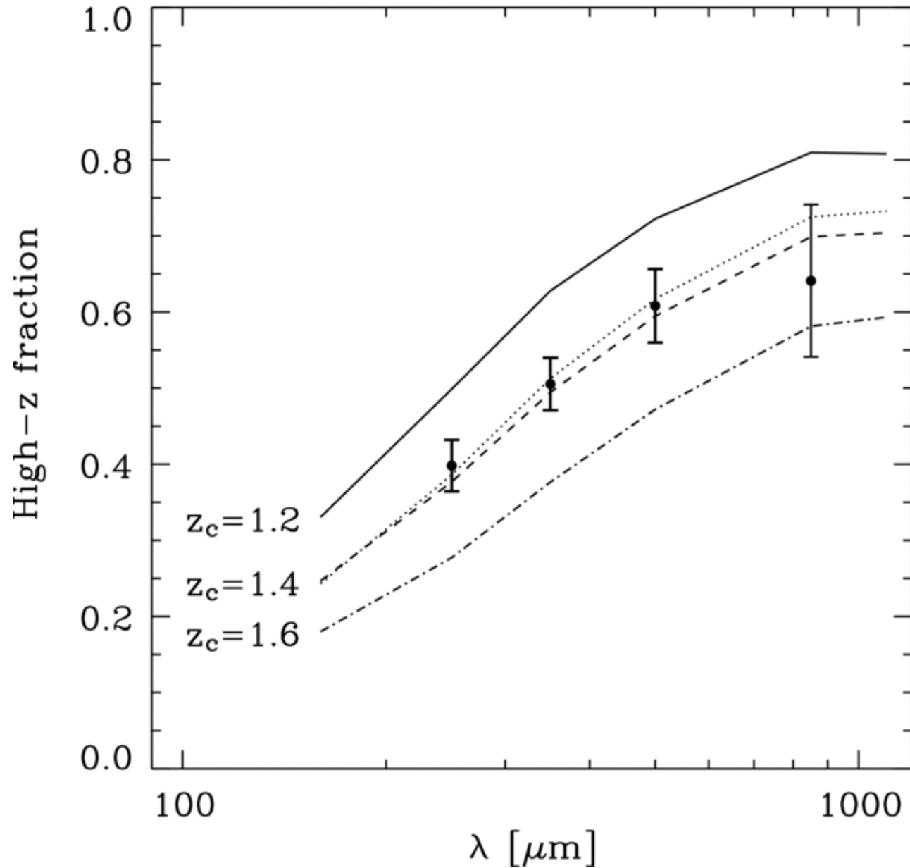
Figure 9. from BLAST: Resolving the Cosmic Submillimeter Background MARSDEN ET AL. 2009 ApJ 707 1729 doi:10.1088/0004-637X/707/2/1729 https://dx.doi.org/10.1088/0004-637X/707/2/1729 © 2009. The American Astronomical Society. All rights reserved.
