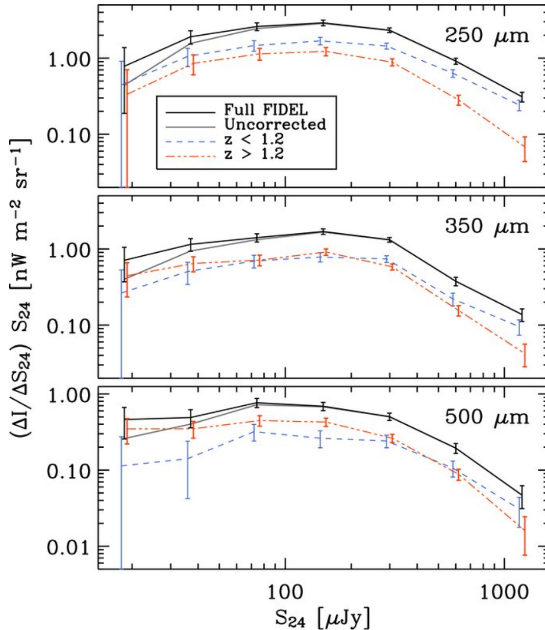
Figure 8. from BLAST: Resolving the Cosmic Submillimeter Background MARSDEN ET AL. 2009 ApJ 707 1729 doi:10.1088/0004-637X/707/2/1729 https://dx.doi.org/10.1088/0004-637X/707/2/1729 © 2009. The American Astronomical Society. All rights reserved.
