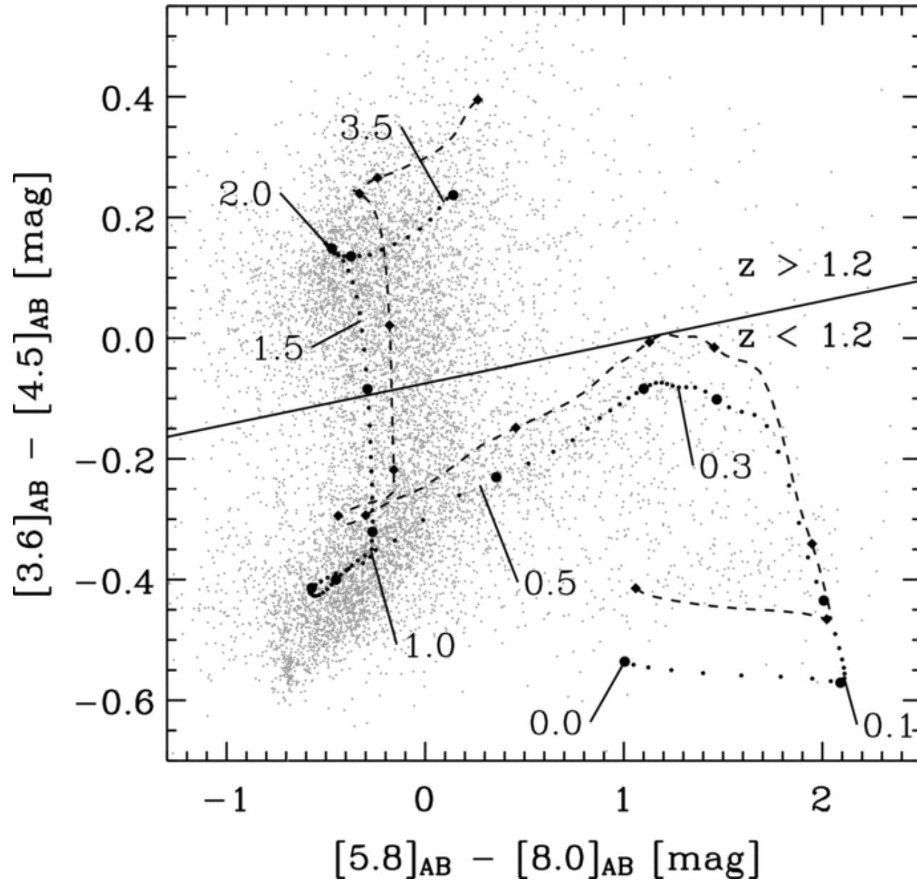
Figure 7. from BLAST: Resolving the Cosmic Submillimeter Background MARSDEN ET AL. 2009 ApJ 707 1729 doi:10.1088/0004-637X/707/2/1729 https://dx.doi.org/10.1088/0004-637X/707/2/1729 © 2009. The American Astronomical Society. All rights reserved.
