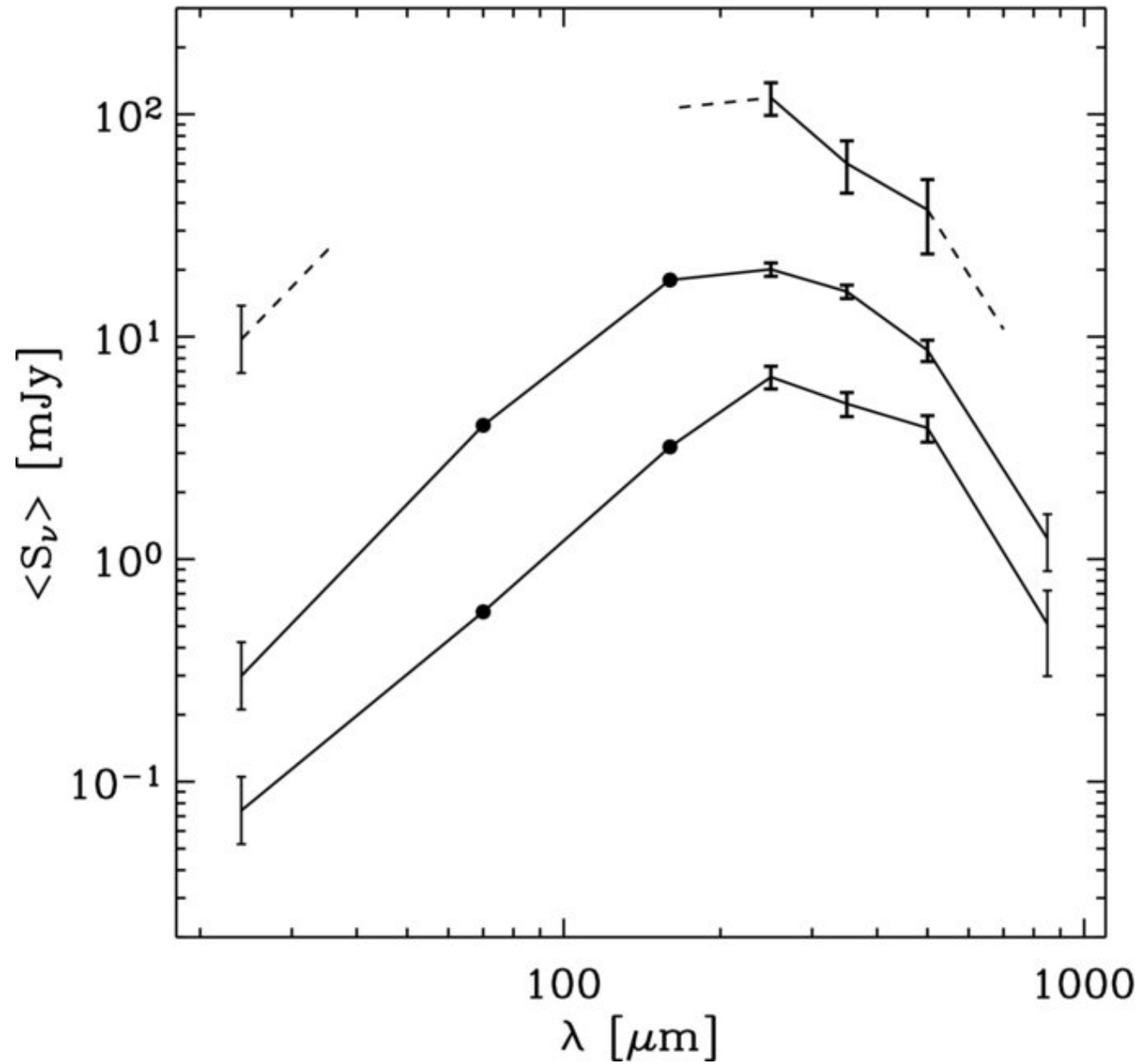
Figure 6. from BLAST: Resolving the Cosmic Submillimeter Background MARSDEN ET AL. 2009 ApJ 707 1729 doi:10.1088/0004-637X/707/2/1729 https://dx.doi.org/10.1088/0004-637X/707/2/1729 © 2009. The American Astronomical Society. All rights reserved.
