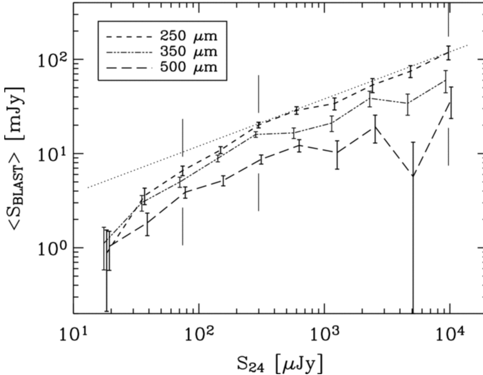
Figure 5. from BLAST: Resolving the Cosmic Submillimeter Background MARSDEN ET AL. 2009 ApJ 707 1729 doi:10.1088/0004-637X/707/2/1729 https://dx.doi.org/10.1088/0004-637X/707/2/1729 © 2009. The American Astronomical Society. All rights reserved.
