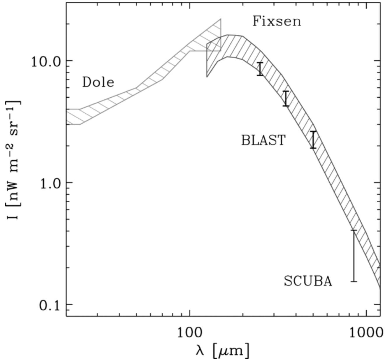
Figure 4. from BLAST: Resolving the Cosmic Submillimeter Background MARSDEN ET AL. 2009 ApJ 707 1729 doi:10.1088/0004-637X/707/2/1729 https://dx.doi.org/10.1088/0004-637X/707/2/1729 © 2009. The American Astronomical Society. All rights reserved.
