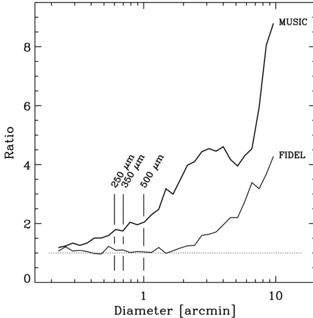
Figure 3. from BLAST: Resolving the Cosmic Submillimeter Background MARSDEN ET AL. 2009 ApJ 707 1729 doi:10.1088/0004-637X/707/2/1729 https://dx.doi.org/10.1088/0004-637X/707/2/1729 © 2009. The American Astronomical Society. All rights reserved.
