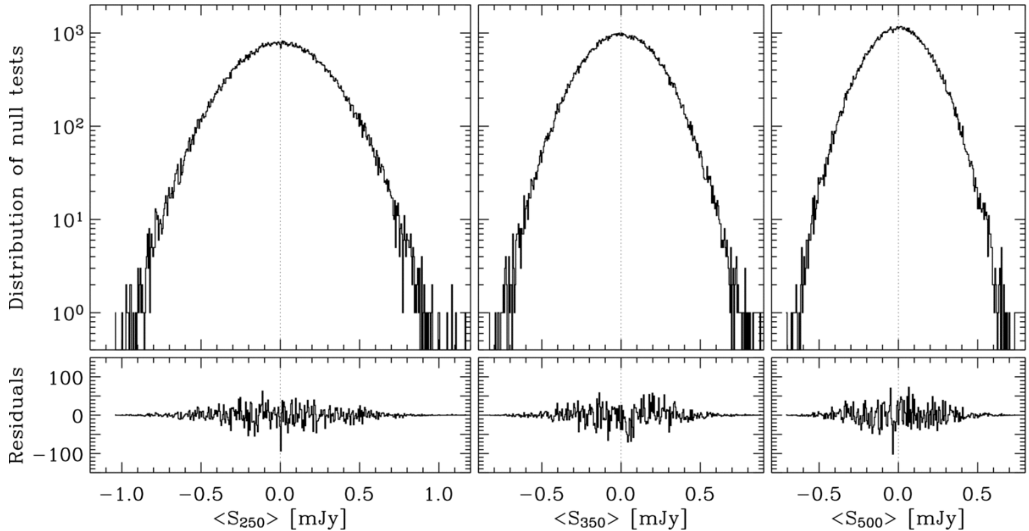
Figure 2. from BLAST: Resolving the Cosmic Submillimeter Background MARSDEN ET AL. 2009 ApJ 707 1729 doi:10.1088/0004-637X/707/2/1729 https://dx.doi.org/10.1088/0004-637X/707/2/1729 © 2009. The American Astronomical Society. All rights reserved.
