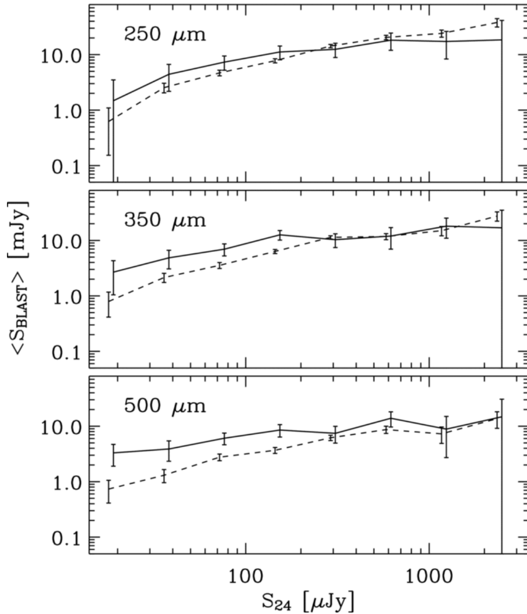
Figure 10. from BLAST: Resolving the Cosmic Submillimeter Background MARSDEN ET AL. 2009 ApJ 707 1729 doi:10.1088/0004-637X/707/2/1729 https://dx.doi.org/10.1088/0004-637X/707/2/1729 © 2009. The American Astronomical Society. All rights reserved.
