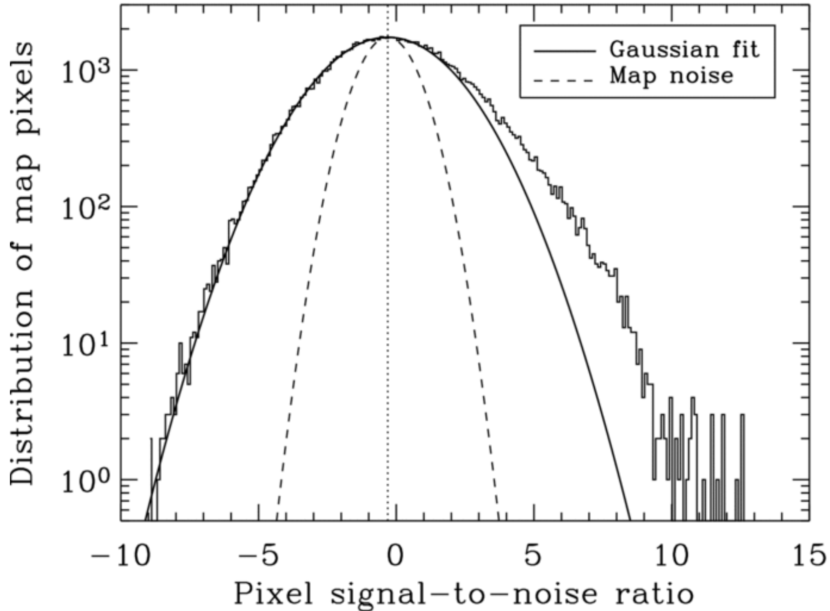
Figure 1. from BLAST: Resolving the Cosmic Submillimeter Background MARSDEN ET AL. 2009 ApJ 707 1729 doi:10.1088/0004-637X/707/2/1729 https://dx.doi.org/10.1088/0004-637X/707/2/1729 © 2009. The American Astronomical Society. All rights reserved.
