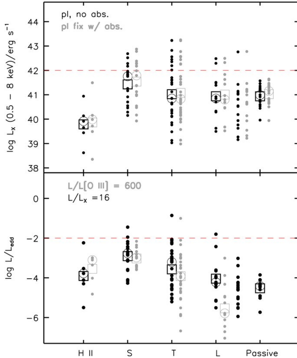
Figure 5. from Probing the Balance of AGN and Star-forming Activity in the Local Universe with ChaMP CONSTANTIN ET AL. 2009 ApJ 705 1336 doi:10.1088/0004-637X/705/2/1336 https://dx.doi.org/10.1088/0004-637X/705/2/1336 © 2009. The American Astronomical Society. All rights reserved.
