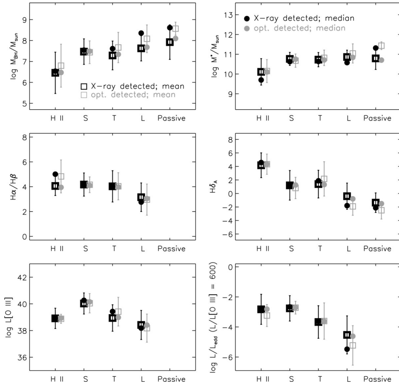
Figure 4. from Probing the Balance of AGN and Star-forming Activity in the Local Universe with ChaMP CONSTANTIN ET AL. 2009 ApJ 705 1336 doi:10.1088/0004-637X/705/2/1336 https://dx.doi.org/10.1088/0004-637X/705/2/1336 © 2009. The American Astronomical Society. All rights reserved.
