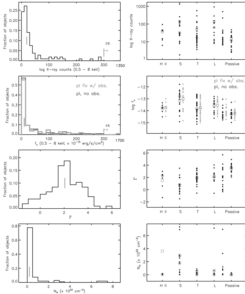
Figure 3. from Probing the Balance of AGN and Star-forming Activity in the Local Universe with ChaMP CONSTANTIN ET AL. 2009 ApJ 705 1336 doi:10.1088/0004-637X/705/2/1336 https://dx.doi.org/10.1088/0004-637X/705/2/1336
