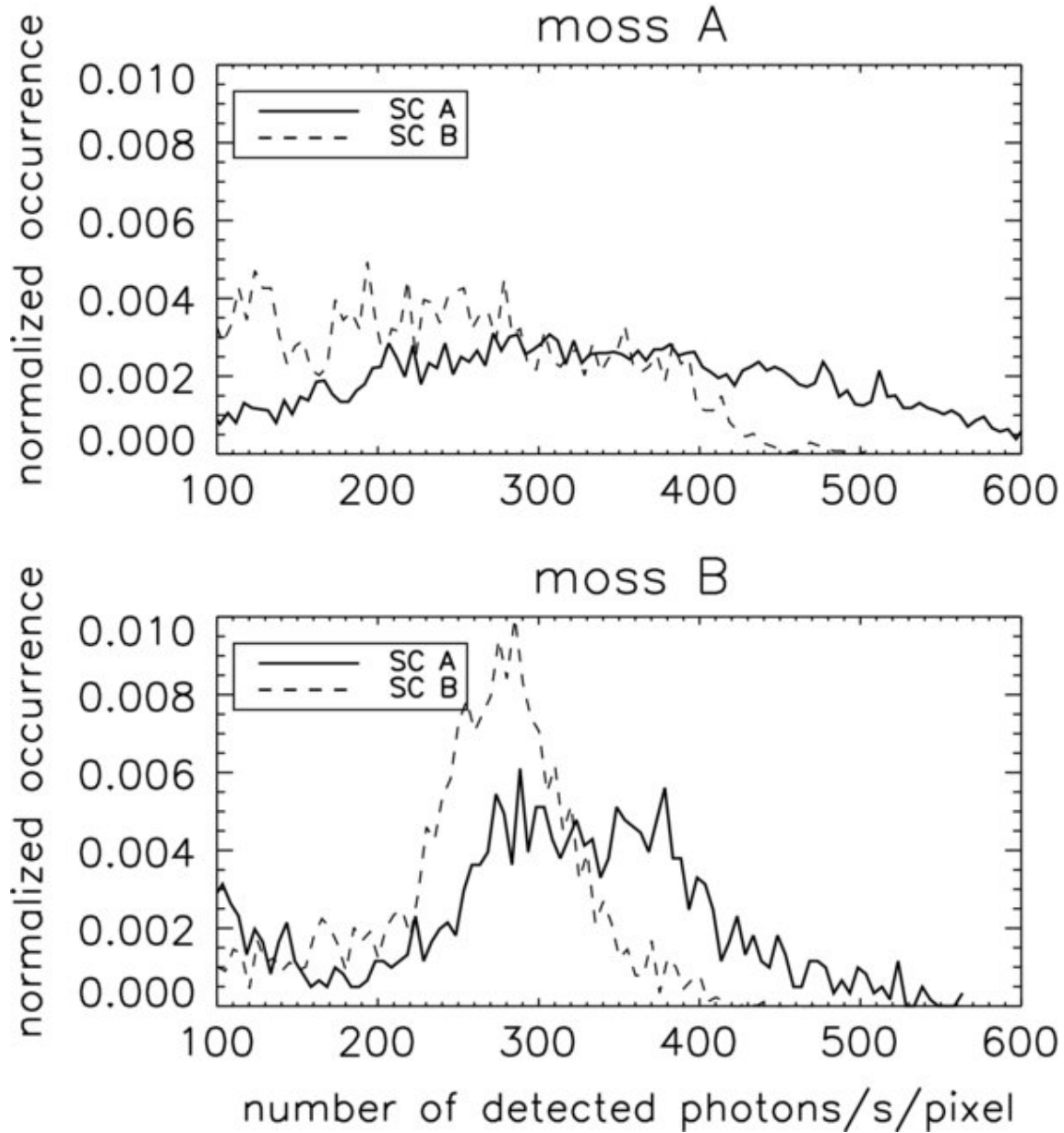
Figure 6. from Estimating the Chromospheric Absorption of Transition Region Moss Emission De PONTIEU ET AL. 2009 ApJ 702 1016 doi:10.1088/0004-637X/702/2/1016 https://dx.doi.org/10.1088/0004-637X/702/2/1016 © 2009. The American Astronomical Society. All rights reserved.
